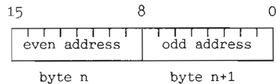
Figure 1. Byte addressing
